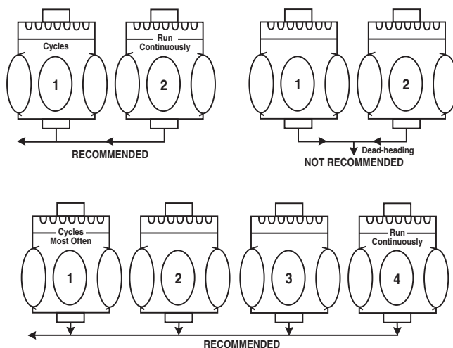
Figure 2 – Discharge Piping
