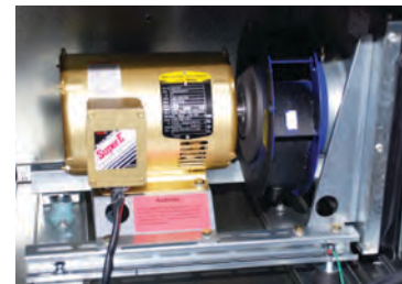
Internally isolated fan and motor
