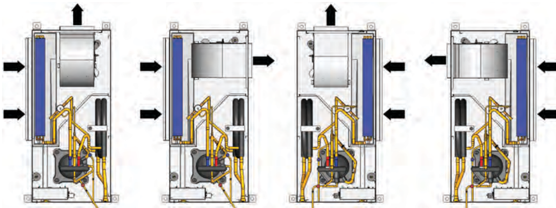
Left-hand return with end discharge
