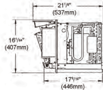
Right End View without Wall Sleeve
