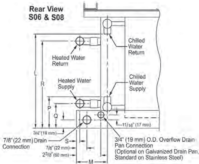
Rear View S16, S20, S30
