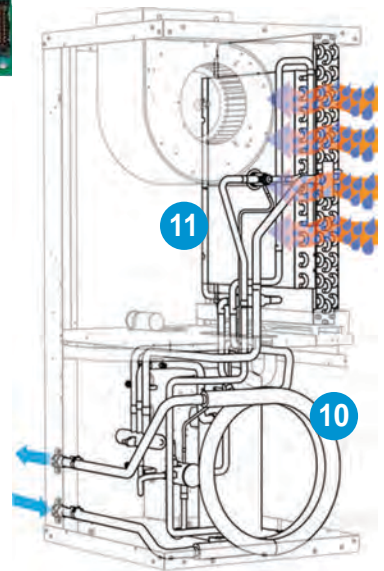
Hot Gas Reheat Coil & Piping Circuit (optional)
